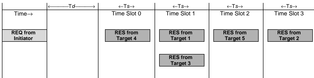
Figure 19: Single Device Detection by Time Slot
