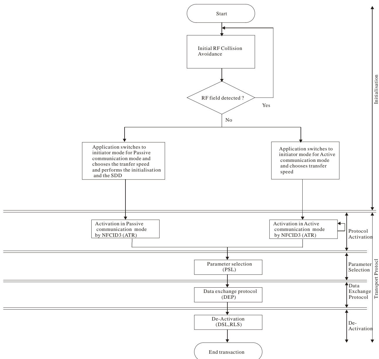
Figure 5: General initialization and single device detection flow
