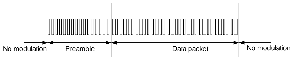
Figure 16: Start and end of communication
