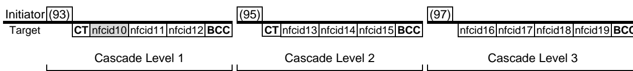
Figure 14: Usage of cascade levels
