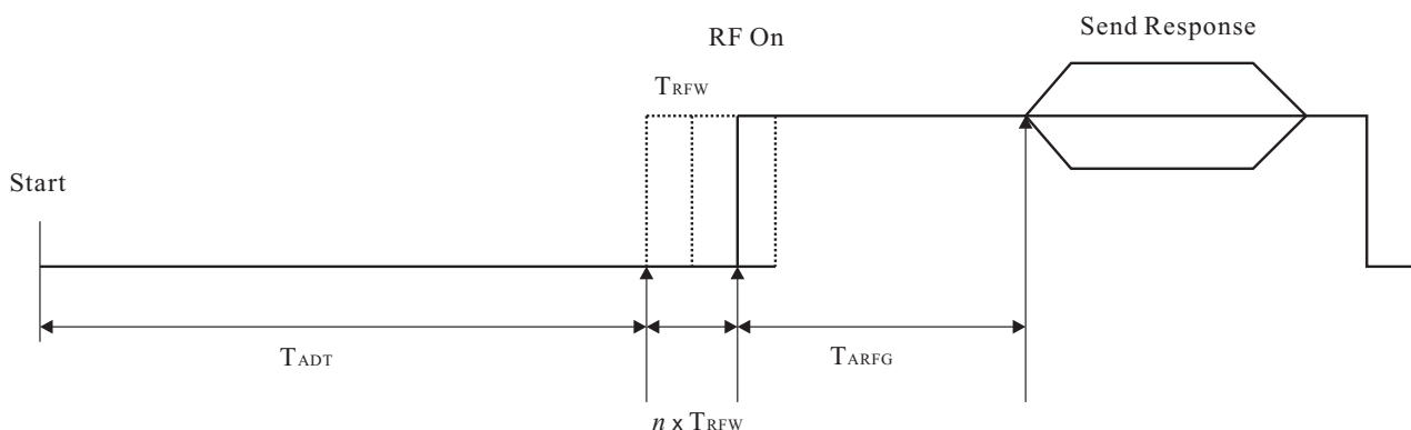
Figure 7: Response RF Collision Avoidance sequence during activation
