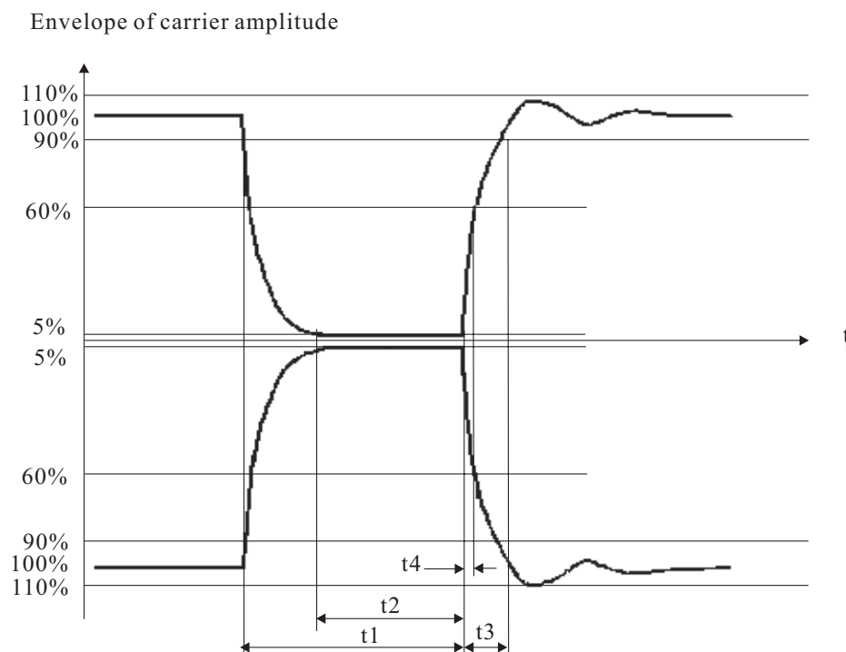
Figure 1: Pulse shape
