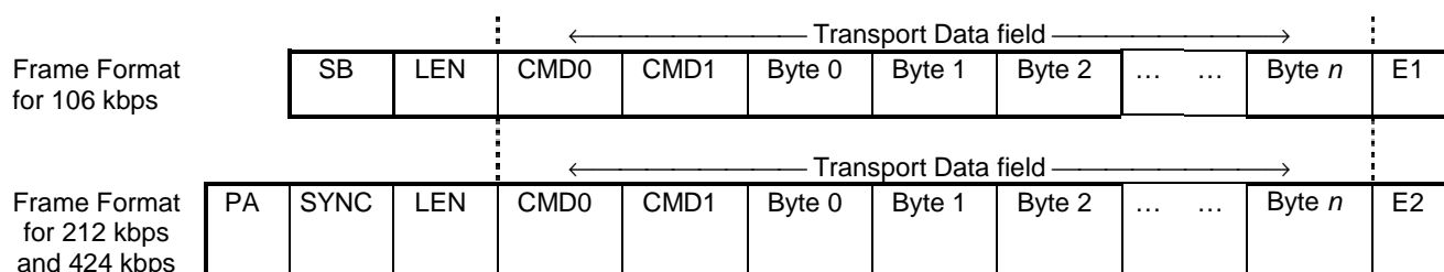
Figure 23: Transport Frame format Definition
