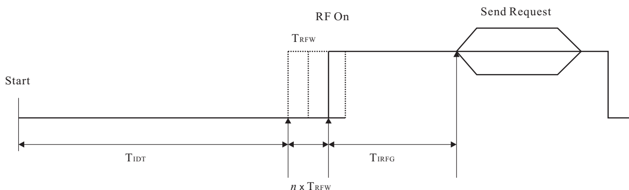
Figure 6: Initial RF Collision Avoidance
